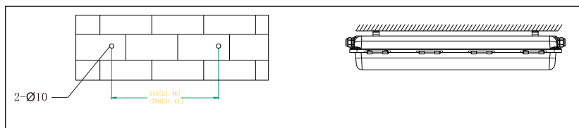
Surface Mount
