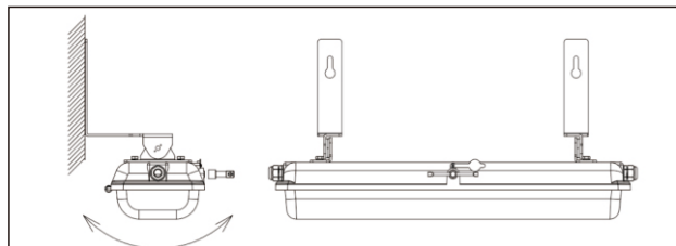
Wall Mount
